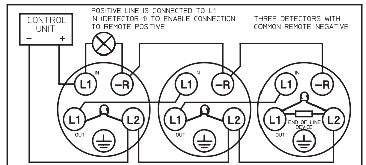
Schematic Wiring Diagram of S60 Monitored Detector Circuit With a Common Remote Indicator Note: Polarity Should be Observed On Detectors Beyond The One Driving The Remote Indicator Earth Terminal is Provided for Easier Installation. It is Not Required by the Detector head. Refer To Apollo Engineering Product Guide For Full Technical Information APOLLO FIRE DETECTORS LIMITED, 36 BROOKSIDE ROAD, HAVANT, P09 1JR ENGLAND
