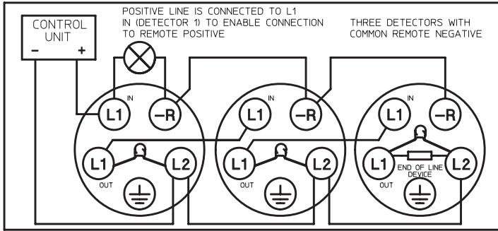
Schematic Wiring Diagram of S60 Monitored Detector Circuit With a Common Remote Indicator Note: Polarity Should be Observed On Detectors Beyond The One Driving The Remote Indicator Earth Terminal is Provided for Easier Installation. It is Not Required by the Detector head. Refer To Apollo Engineering Product Guide For Full Technical Information APOLLO FIRE DETECTORS LIMITED, 36 BROOKSIDE ROAD, HAVANT, P09 1JR ENGLAND
