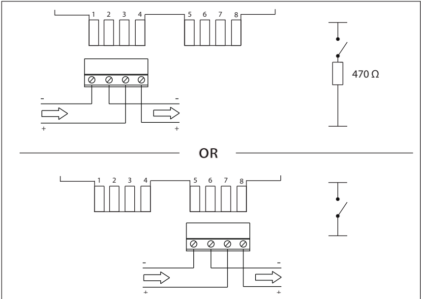
Fig 2 Terminal block connections
